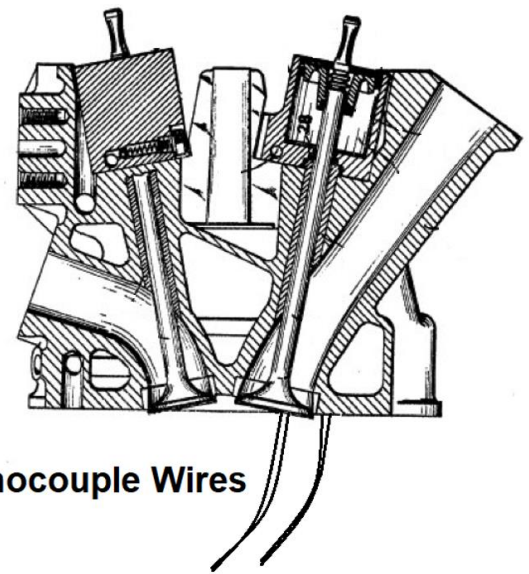
Figure 4. The procedure for thermocouple insertion and exiting the thermocouple wires
